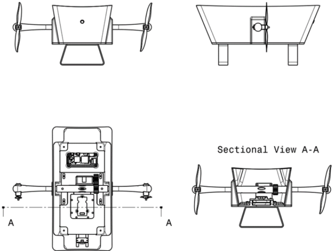
Figure 37: Detailed structural draft of the improved blimp
