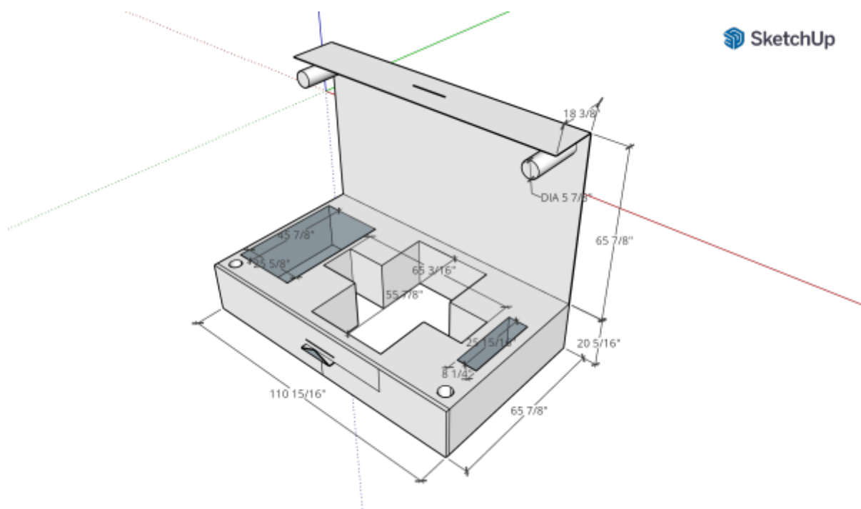
Figure 65: Packaging Model
