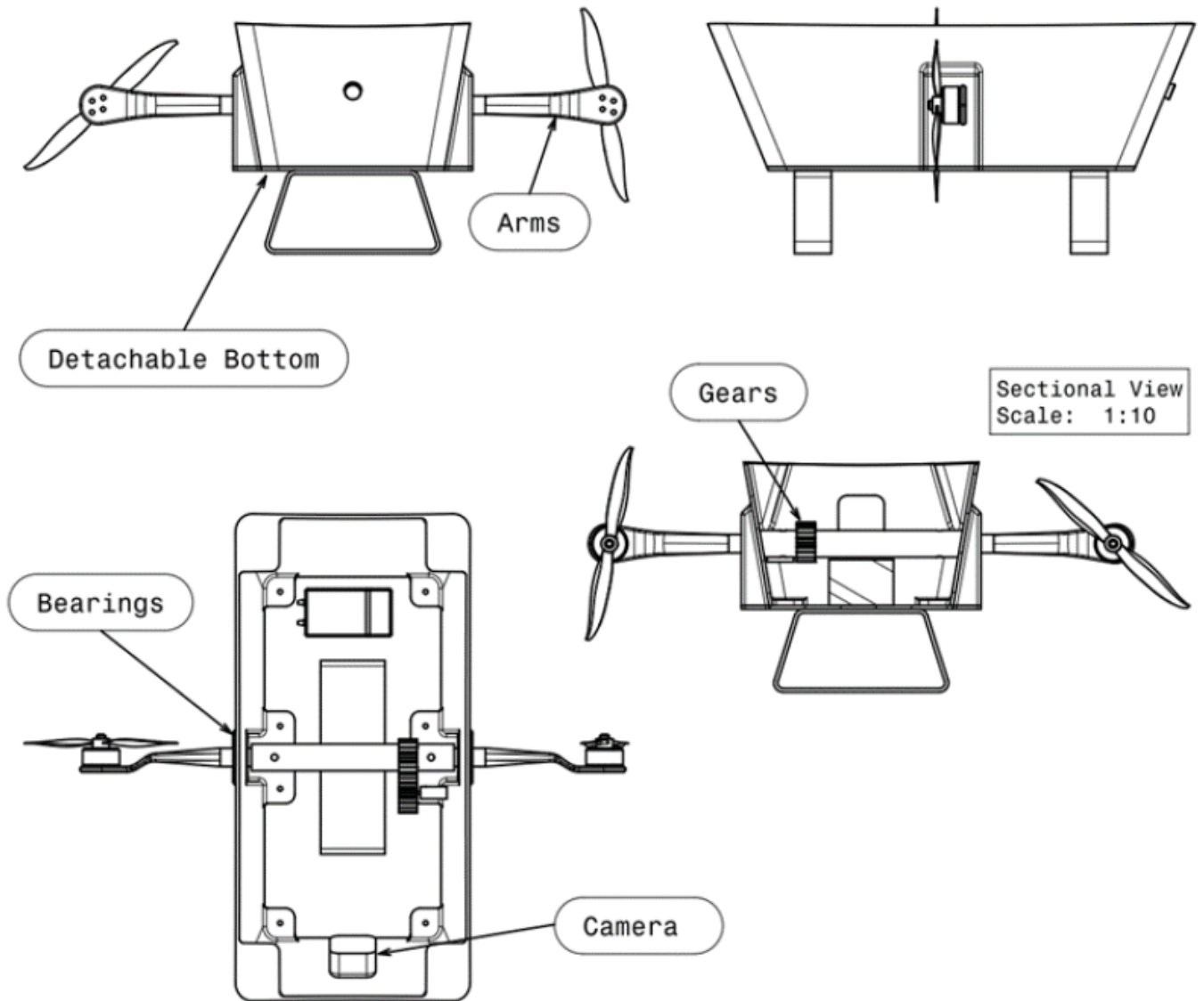
Figure 36: Detailed structural draft
