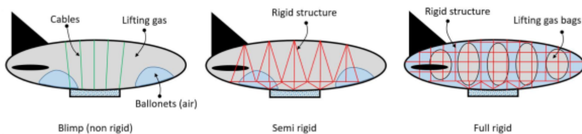
Figure 4: Blimp structure [Durga Vasudevan, Hariharan Mohan, Saarang Gagar, Ramesh Burela Gupta, 2019]
